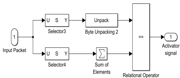
Figure 8: Checksum block
